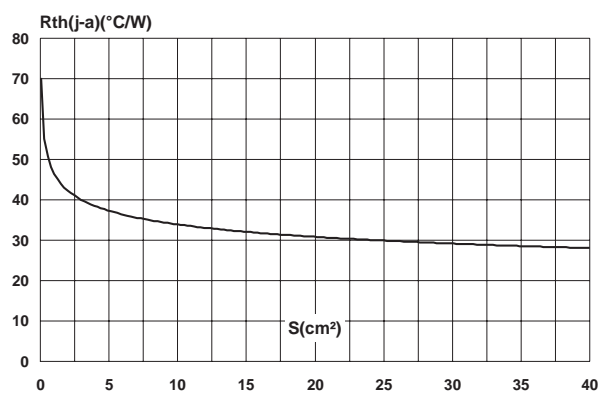
Fig. 8: Thermal resistance junction to ambient versus copper surface under tab (epoxy printed board FR4, \text{Cu} = 35\mu\text{m} ). (STPS41H100CG only)
