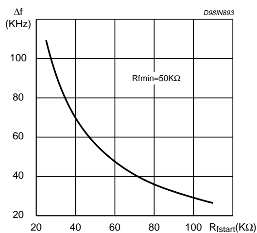
Figure 8. Typ. (f_{start}-f_{min}) vs. R_{fstar} @ C_f = 470\text{pF}
